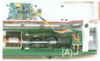
DIGITAL
